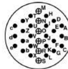
30 Contacts
