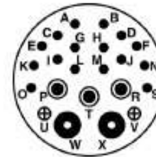
23 Contacts
